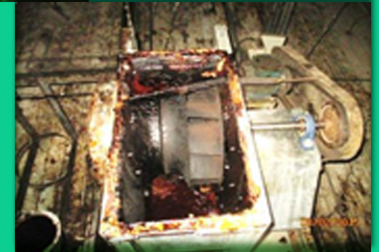
Blower
